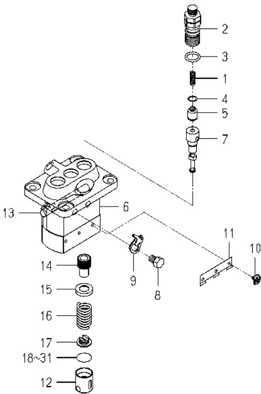
FIG. 29 COMPONENT PARTS FOR 6215-600-103-30 ON Fig.21
