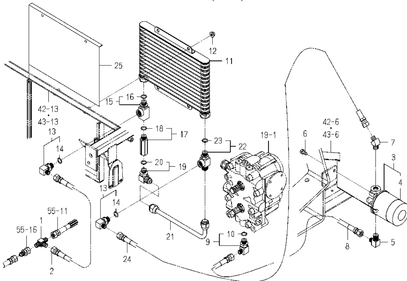
FIG. 56 PIPING(HST)SYSTEM
