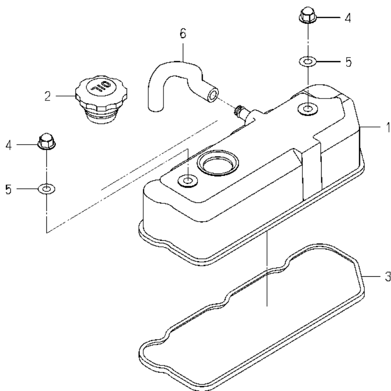
FIG. 3 CYLINDER HEAD COVER
