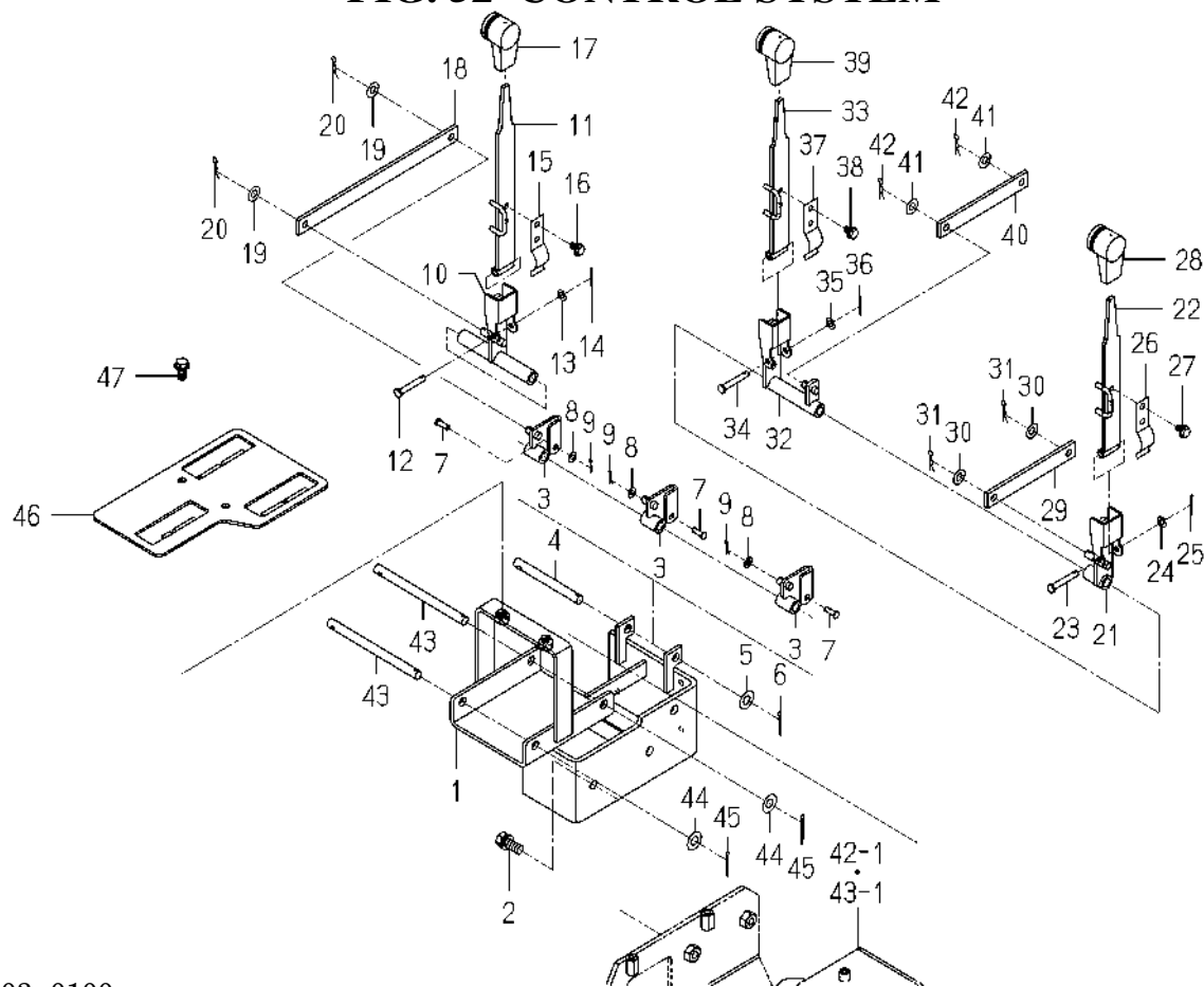
FIG. 52 CONTROL SYSTEM
