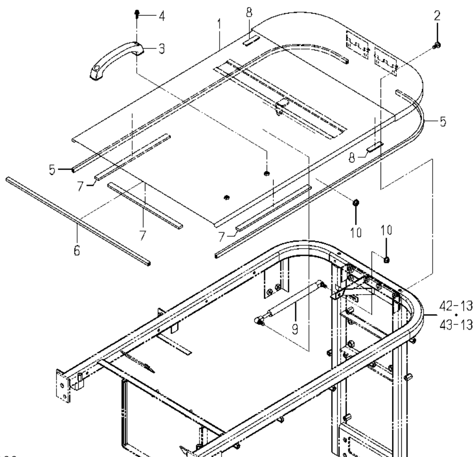
FIG. 58 HOOD SYSTEM
