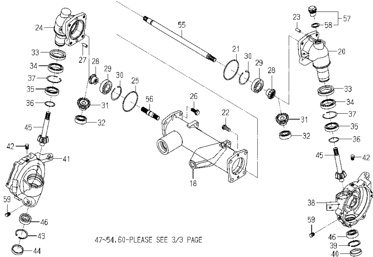
FIG. 49 HOUSING(AXLE/REAR)SYSTEM(2/3)
