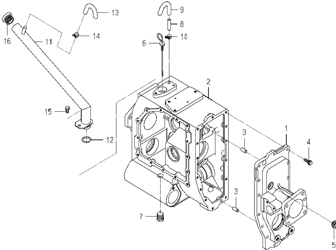
FIG. 16 CASE(TRANSMISSION)SYSTEM
