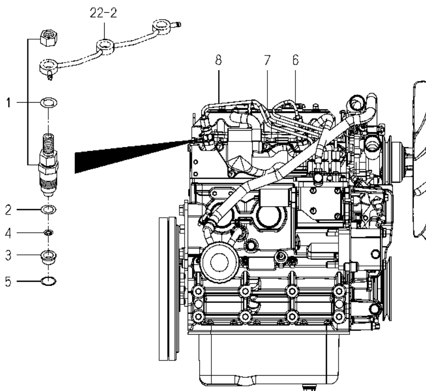
FIG. 20 INJECTION NOZZLE
