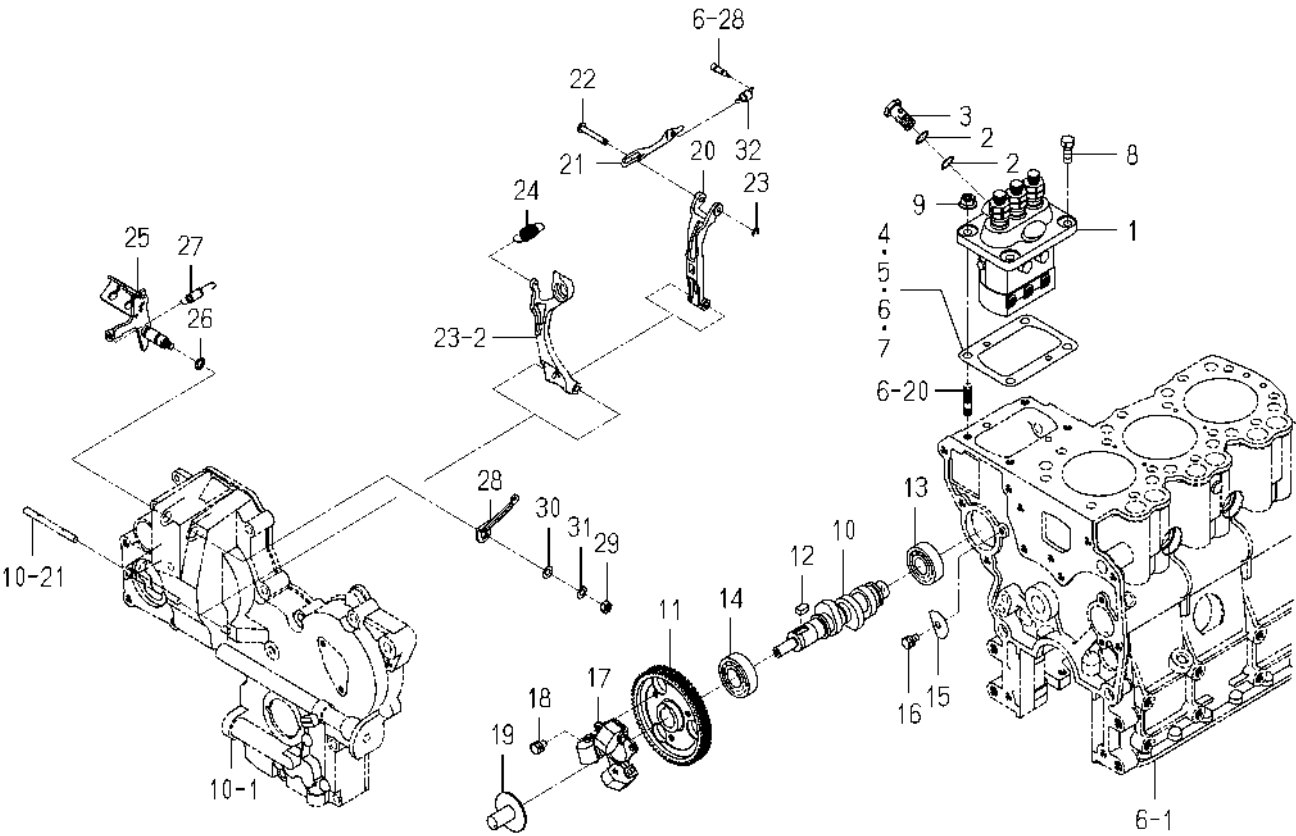
FIG. 21 INJECTION PUMP
