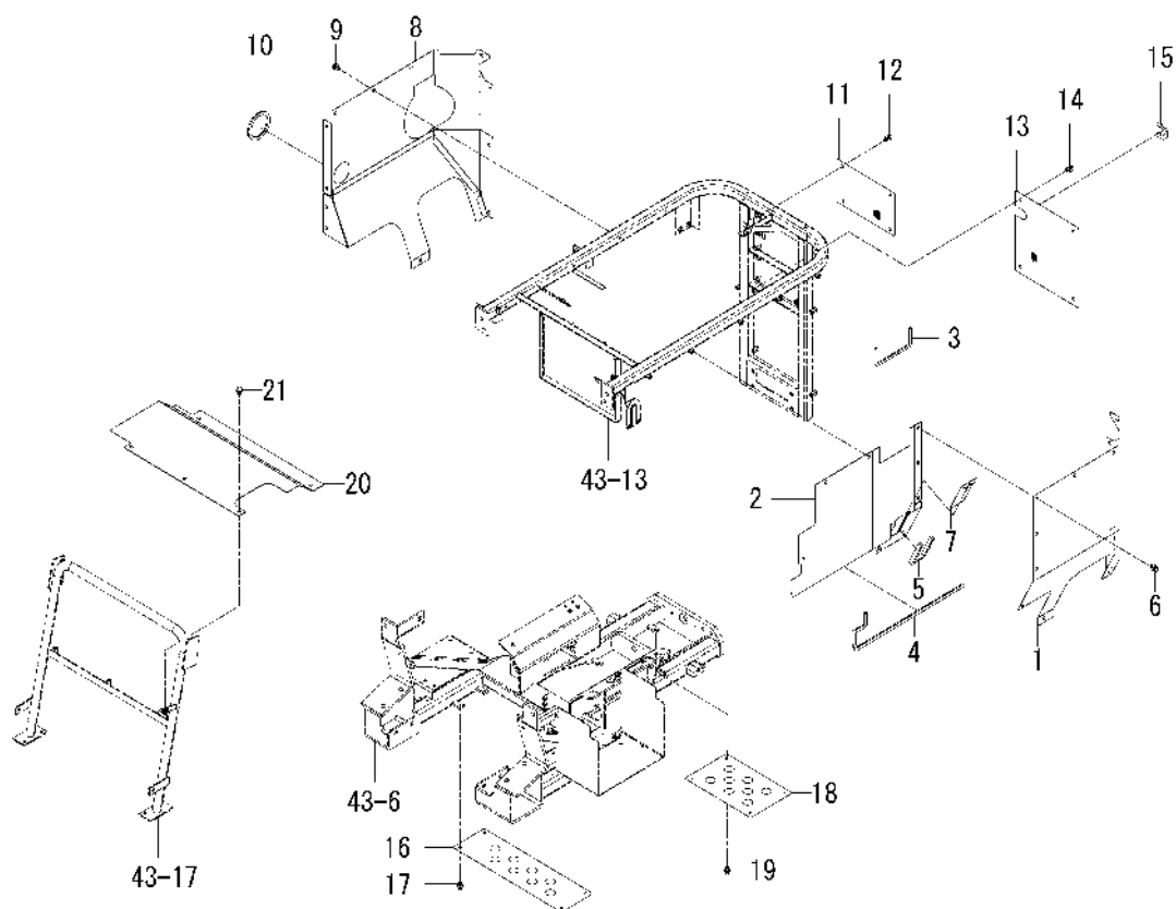
FIG. 45 COVER(SIDE)SYSTEM(EXCEPT B TYPE)
