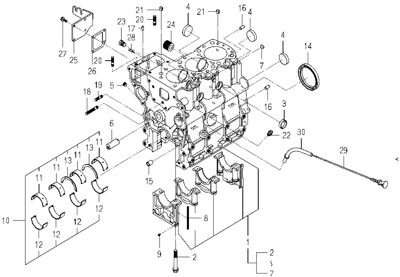
FIG. 6 CYLINDER BLOCK
