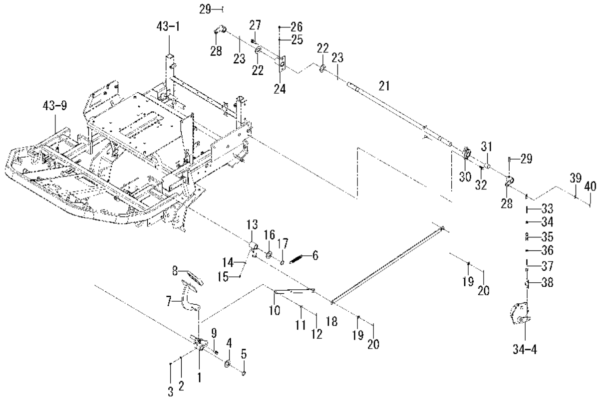
FIG. 35 PEDAL(BRAKE)SYSTEM
