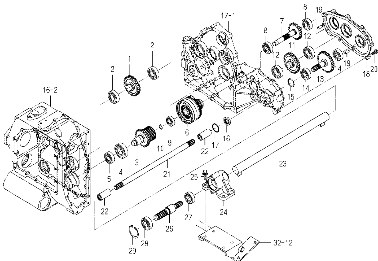
FIG. 26 DRIVE(PTO/SIDE)SYSTEM
