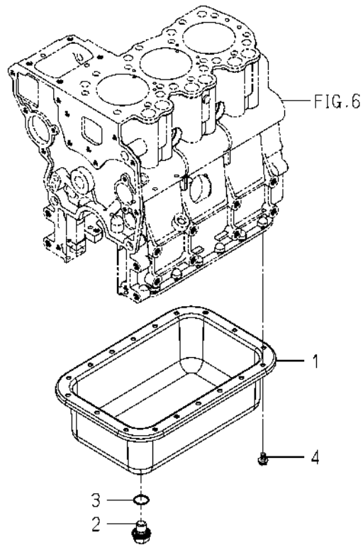
FIG. 8 OIL PAN
