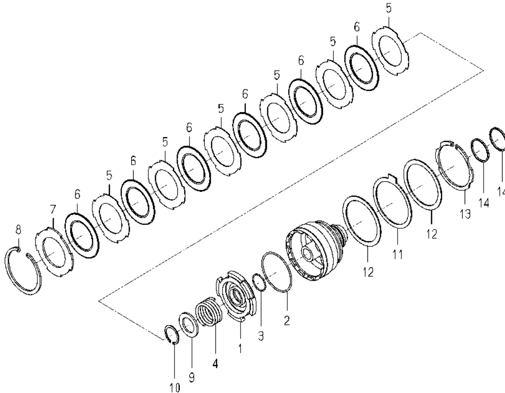
FIG. 87 COMPONENT PARTS FOR 1825-127-300-00 ON Fig.26
