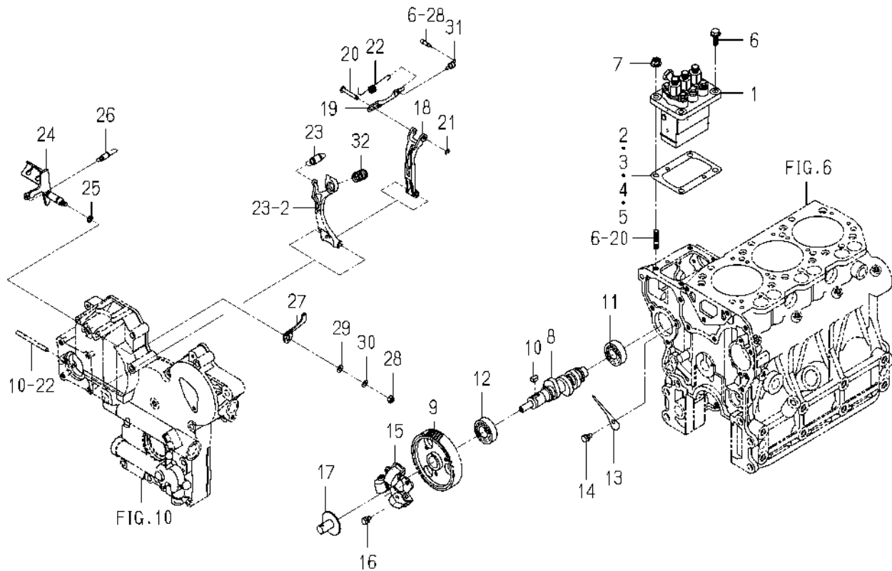
FIG. 21 INJECTION PUMP
