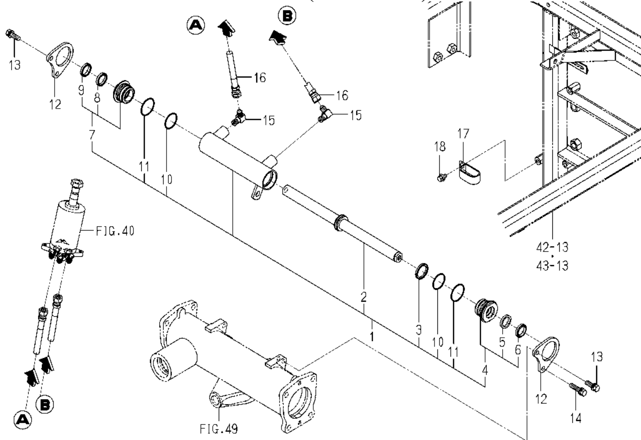
FIG. 41 CYLINDER(STEERING)SYSTEM
