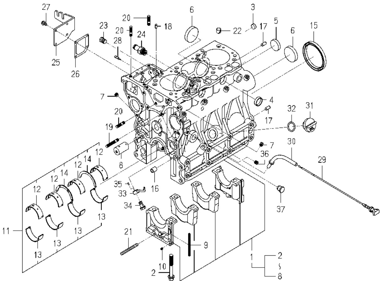
FIG. 6 CYLINDER BLOCK
