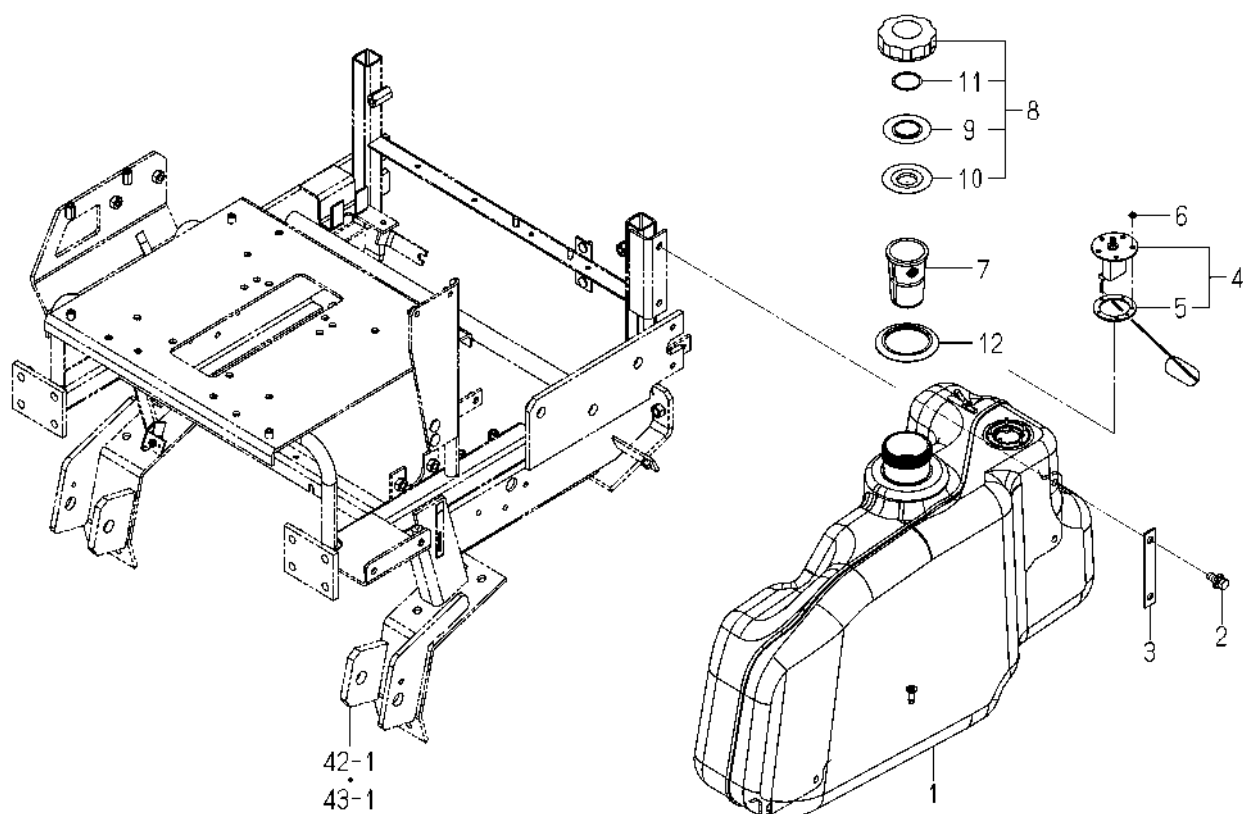
FIG. 10 TANK(FUEL)SYSTEM
