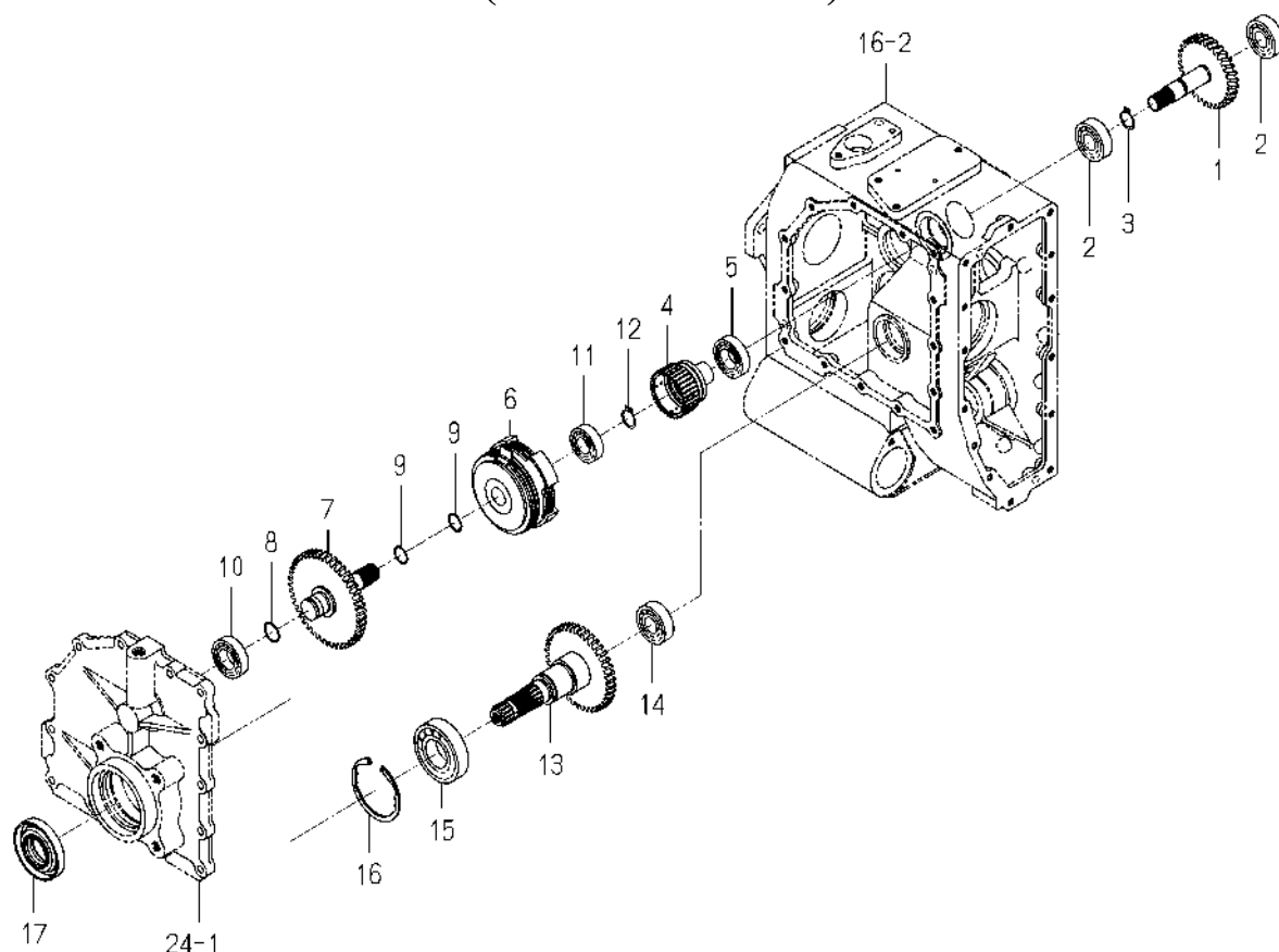
FIG. 27 DRIVE(PTO/BLOWER)SYSTEM (B TYPE SF235F)
