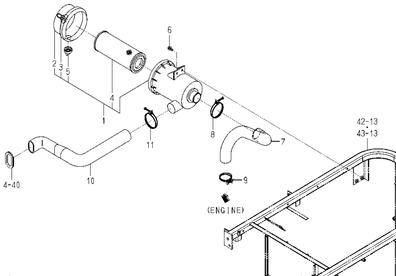
FIG. 8 CLEANER(AIR)SYSTEM(SF224F TYPE)
