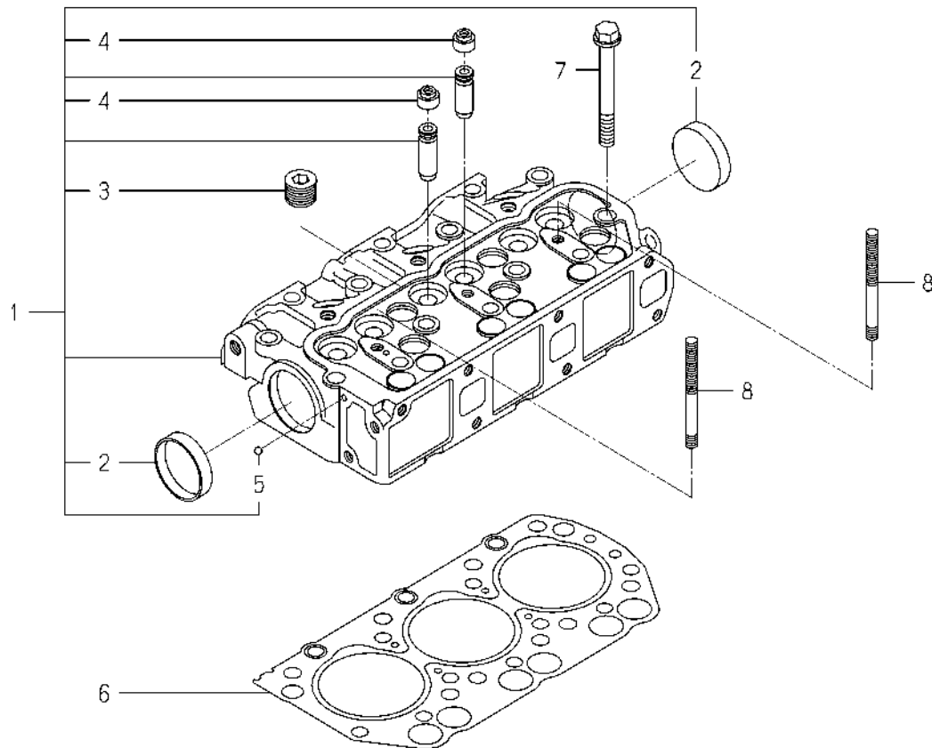
FIG. 2 CYLINDER HEAD
