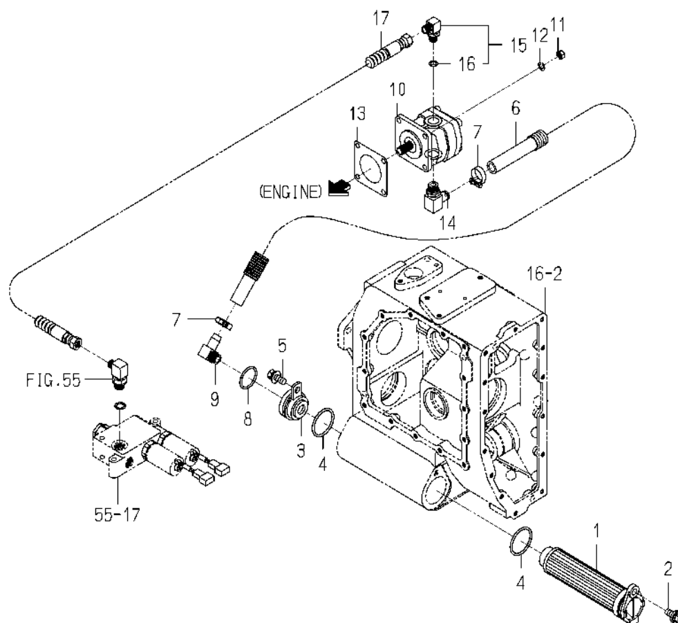
FIG. 54 PIPING(PUMP)SYSTEM
