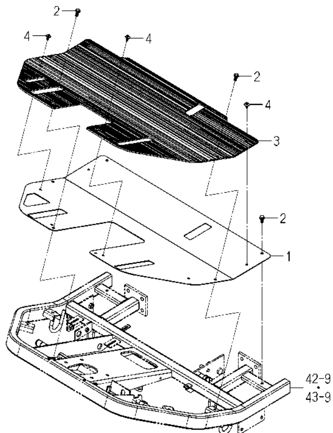
FIG. 62 FLOOR SYSTEM
